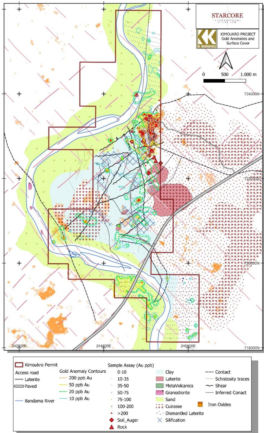
FIGURE 4. Distribution of gold anomaly from soil and rock samples
