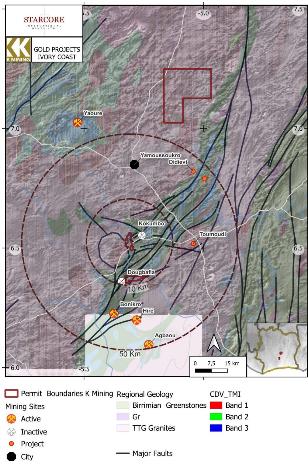
FIGURE 1: Regional geology over shaded TMI magnetic image and major structures
