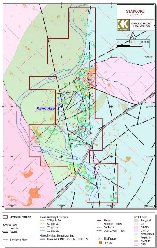
FIGURE 2: Local geology and major structures. Contours of gold anomalies are shown.
