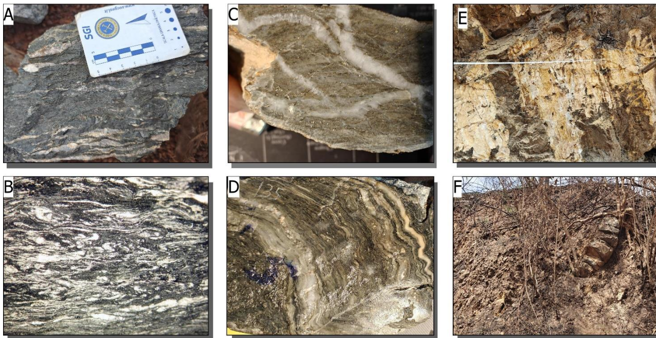
FIGURE 3. Style of quartz-veining and progressive deformation.
